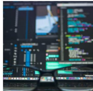
Database design
